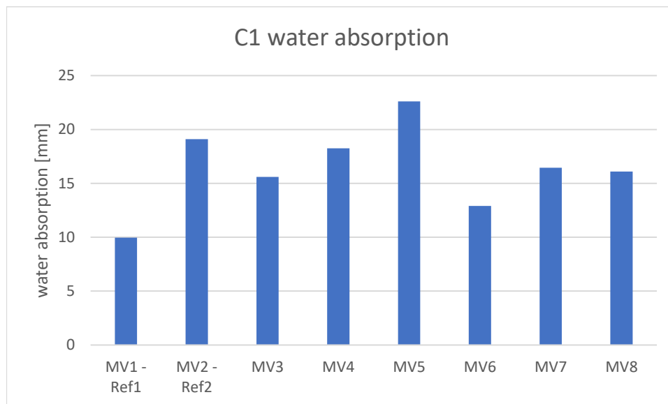
Figure 30 Illustration of the C1 concrete water absorption
