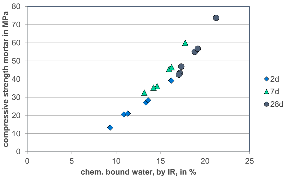
Figure 21 chemical bound water of cement stone correlated with mortar compressive strength
