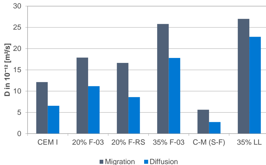
Figure 47 Chloride diffusion and migration coefficients
