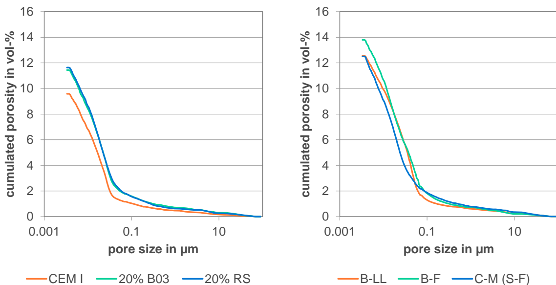
Figure 19 porosity of mortars
